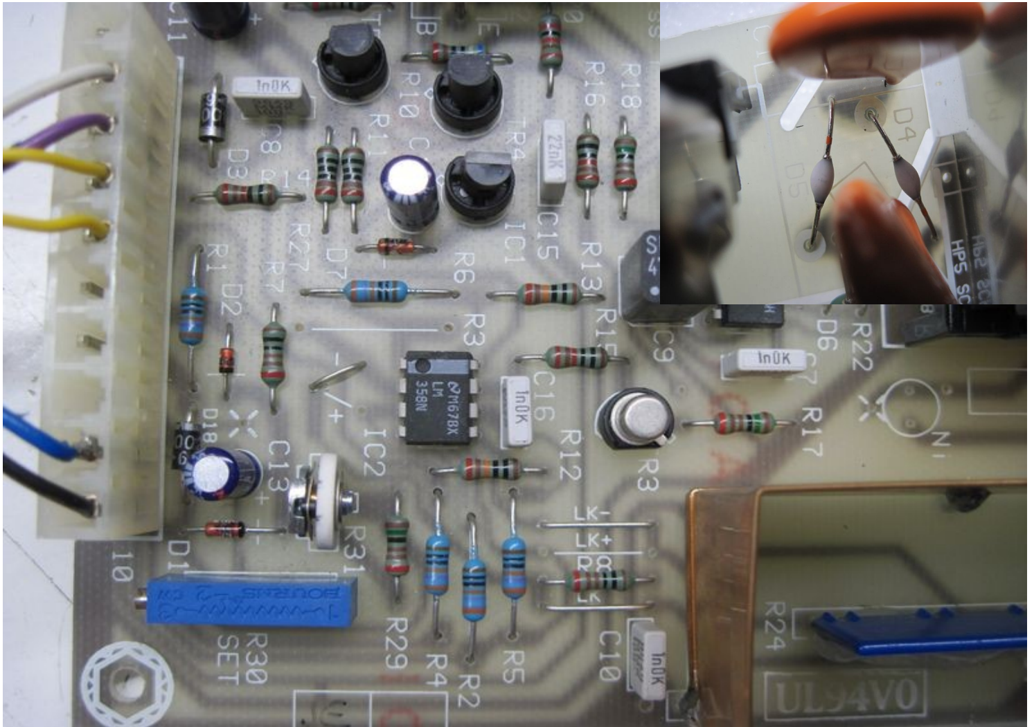
Photo original position of component, HP1N negative HV
